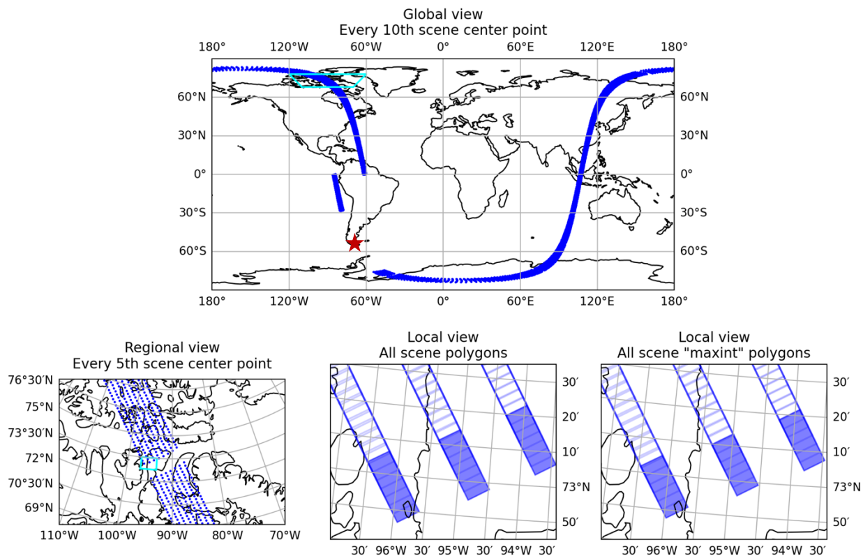
Figure 1-3 shows an example geolocated orbit (top panel) and focused regional and local plots (bottom panels). The global plot was selected to illustrate a data gap due to a data downlink at the Punta Arenas, Chile ground station, from approximately -70^{\circ}\text{S} to -30^{\circ}\text{S} on the ascending pass at the end of the granule. The zoomed in regional view (lower left) shows the data within the small cyan box in the global plot, and illustrates a smaller data gap due to instrument calibration. The local views (lower middle and right) show the actual scene ground footprint polygons, for the cyan box denoted in the regional view. The first scene's polygon is filled blue, to illustrate the shape of the full field of view (FOV) for one data integration. During the 0.7 second integration time, the satellite moves along track slightly more than 5 km, which means the leading and trailing edges of the instantaneous FOV have translated forward by the same amount. The lower right plot shows the "max integration" footprint polygon, which includes the interior portion of the scene footprint that was within the sensor field of view for the entire integration period.
